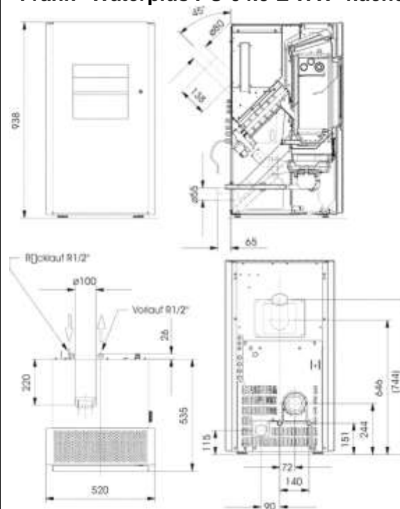
"Frank" Waterplus PO 04.5 E WW- flache Tür
